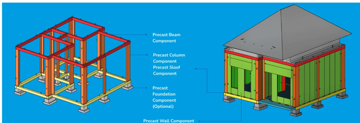
Figure 3. Precast House Panel
